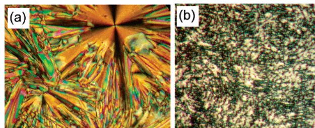
Figure 7. Textures of compound \text{Si}_3\text{-11B18} as seen between crossed polarizers: (a) \text{USmC}_s\text{P}_F phase at 106 °C, as obtained by cooling from the isotropic liquid; (b) \text{USmC}_s\text{P}_F phase at 90 °C as obtained by cooling from the \text{USmC}_s\text{P}_F phase.
