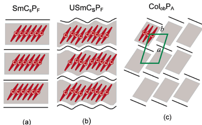
Figure 9. Possible way for the transition from (a) a smectic phase via (b) a nonsinusoidal undulated smectic phase (wavy deformed layers, the undulation period can be much larger than actually shown) to (c) an oblique columnar phase (broken layers, the resulting ribbons are organized in an oblique lattice) as observed with increasing steric frustration. The transition from wavy deformed layers to broken layers is associated with a change of the polar order from ferroelectric to antiferroelectric. The possibilities concerning the polar directions in the \text{Col}_{\text{ob}}\text{P}_A phase are discussed in Figure S6, Supporting Information.
