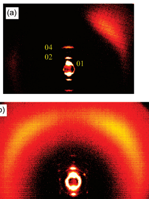
Figure 8. X-ray diffraction pattern of aligned samples. (a) \text{USmC}_s\text{P}_F phase of compound \text{Si}_3\text{-11B18} at 85 °C (the 03 reflection is very weak); the diffraction pattern does not change at the transition to the \text{USmC}_s\text{P}_F phase; (b) \text{ColobP}_A phase of \text{Si}_3\text{-11B22} at 97 °C; in both cases, the stronger intensity of the wide-angle scattering on the right is indicative of a synclincic tilt of the molecules; in (b), synclincic domains with opposite tilt direction coexist, and therefore, a wide-angle scattering is also found on the left; the distinct intensity of these scatterings indicates a synclincic organization, but if both would have the same intensity, a synclincic or anticlincic tilted organization could not be distinguished.
