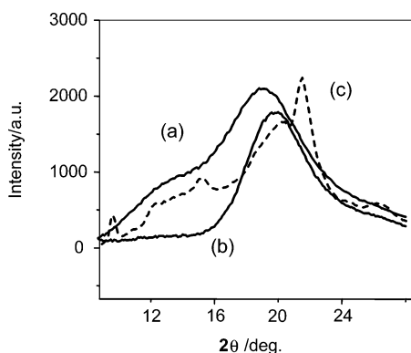
Figure 4. Wide-angle region of selected X-ray diffraction pattern: (a) two diffuse maxima in the \text{SmC}_s\text{P}_F^{[38]} phase of compound \text{Si}_3\text{-11B14} at 100 °C indicate a nanosegregated structure with discrete oligosiloxane sublayers; (b) one diffuse maximum in the \text{USmC}_s\text{P}'_F phase of compound \text{Si}_3\text{-11B18} at 92 °C indicates the absence of separate oligosiloxane sublayers; (c) several reflections in the \text{SmX}^{[8]} phase of compound \text{Si}_3\text{-11B14} at 50 °C indicate an additional in-plane order.
