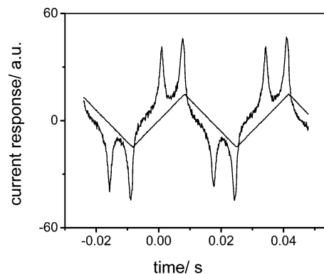
Figure 14. Switching current response of the \text{Col}_{ob}\text{P}_A phase of compound Si 3 -11B22 in a 5\ \mu\text{m} noncoated ITO cell ( \pm 150 V, 20 Hz) at T = 90\ ^\circ\text{C} .
