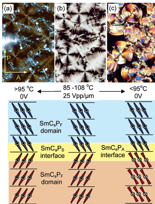
Figure 13. Temperature dependence of the switching process of compound Si 3 -11B18 , (b) under the applied AC field (6 \mu\text{m} polyimide-coated ITO cell, 25 \text{V}_{pp}/\mu\text{m} , f = 1 Hz); (a) after switching off the field at T > 95 °C, the position of the dark extinction brushes does not change (FE state is stable at the surfaces and in the center of the cell relaxes to a dark conglomerate phase); and (c) after switching off the field at T < 95 °C, in the bright regions the dark brushes become inclined with respect to polarizer and analyzer (the FE state relaxes to the AF ground state by rotation on a cone); in the dark regions, the texture is the same as in (a); the models below show sections of the proposed microdomain structures composed of \text{SmC}_s\text{P}_F domains with synpolar and anticlinic interfaces in (a) and (b) and with antipolar and synclinc interfaces in (c); to avoid confusion the terms synpolar (subscript S) and antipolar (subscript A) are used to characterize the polar correlation between domains, whereas the polar correlation between the individual layers is described as ferroelectric (= synpolar) and antiferroelectric (= antipolar).
