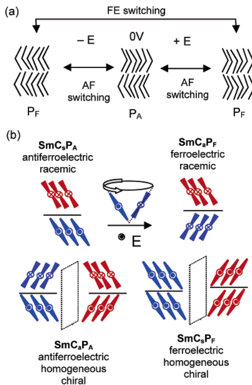
Figure 1. (a) The switching of bent-core molecules (side views) and (b) the four possible arrangements in tilted polar smectic phases. The subscripts 's' and 'a' indicate the correlation of the tilt direction in adjacent layers: s = synclinal means an identical tilt direction; a = anticlinal indicates an opposite tilt direction. Subscripts 'A' and 'F' indicate the correlation of the polar direction in adjacent layers. \text{P}_A is indicative of an antipolar structure (polar direction alternates); this structure is macroscopically nonpolar and usually assigned as antiferroelectric. \text{P}_F stands for a synpolar structure (polar direction is identical); this structure is macroscopically polar and usually assigned as ferroelectric (and therefore abbreviated as \text{P}_F ). The color indicates the chirality of the layers ( superstructural chirality; for details, see Figure S1 in Supporting Information). The \text{SmC}_a\text{P}_A and \text{SmC}_s\text{P}_F structures are homogeneous chiral (identical chirality sense in the layers), and the \text{SmC}_s\text{P}_A and \text{SmC}_a\text{P}_F structures are macroscopic racemic (alternating chirality sense in the layers). Switching usually takes place on a cone (shown in the middle). It reverses polar direction and tilt direction and retains the layer chirality.
